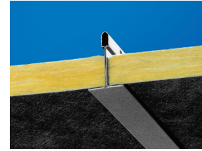
Section of Sombra A system
