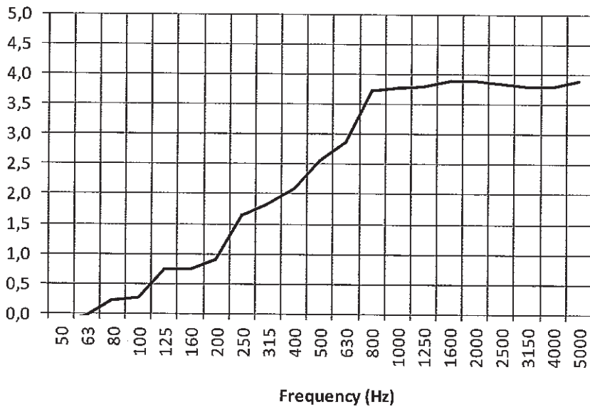
Equivalent sound absorption area (m 2 Sabine).
