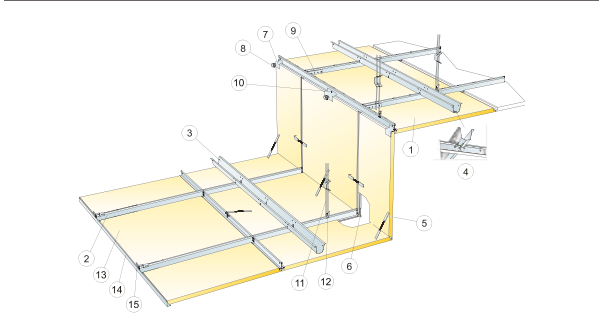
M394 Installation diagram (M394) for Ecophon Focus Ds Levelchange
