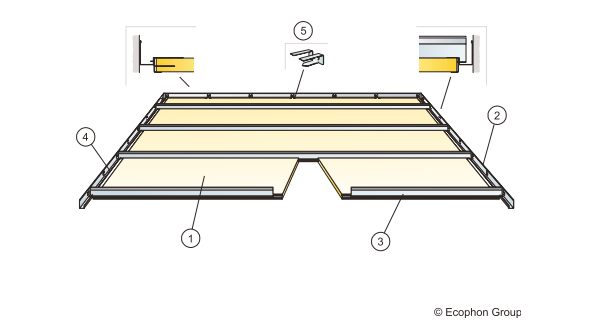
M400 Installation diagram (M400) for Ecophon Focus Ds
