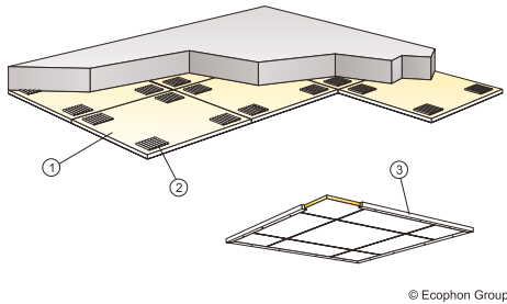
M03 Installation diagram (M03) for Ecophon Focus B, using Connect Absorber glue
