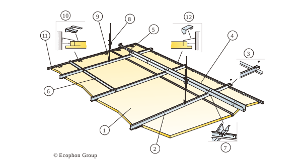
M206 Installation diagram (M206) for Ecophon Focus Ds 600x600, 1200x600 mm and Ecophon Focus Ds XL. Suspended installation
