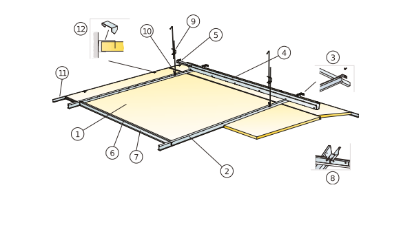
M207 Installation diagram (M207) for Ecophon Focus Ds 1200x1200 mm
