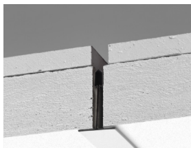
Detail systému Combison Duo A
